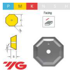
YG1 OFER070405-YG602 PLACA DE FRESAR
